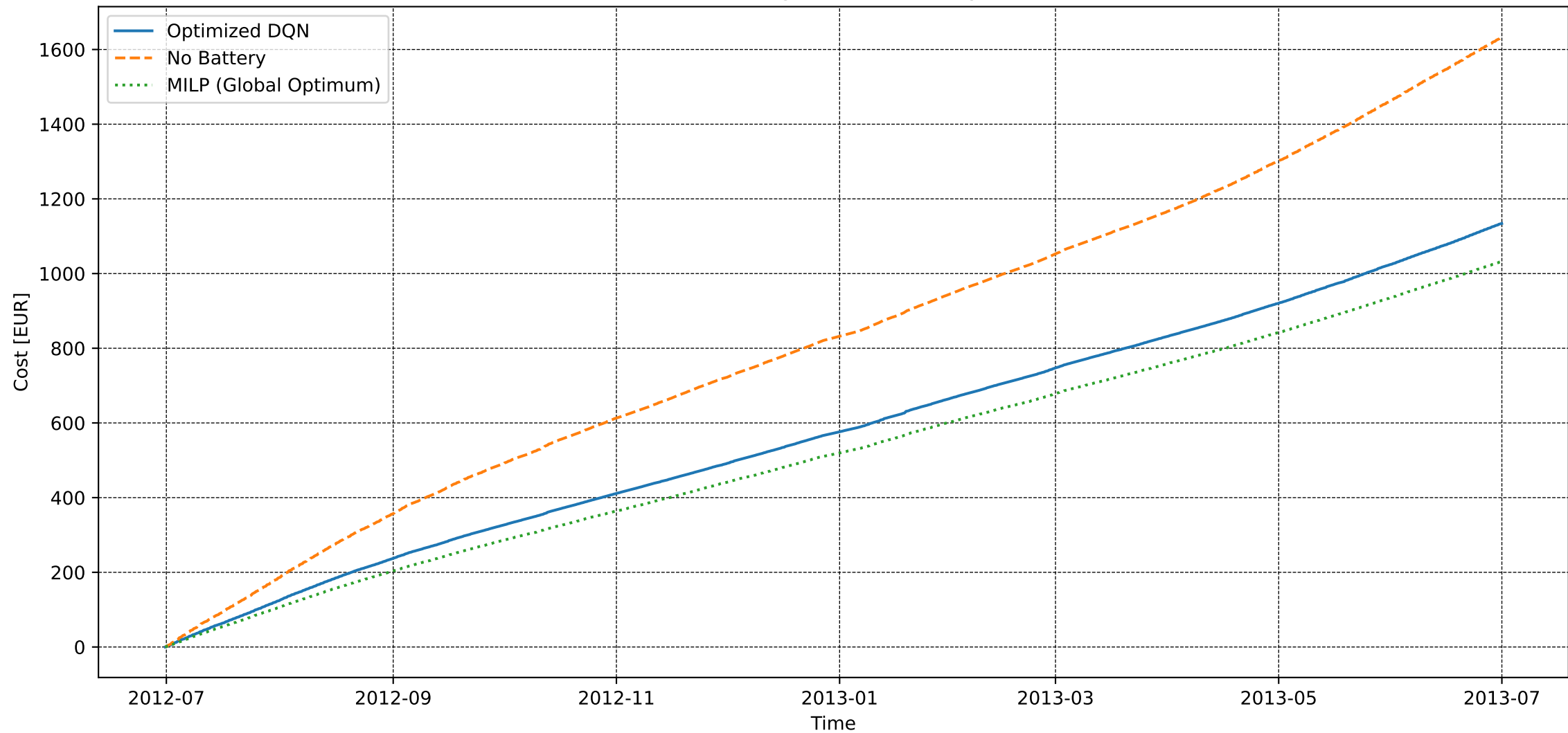
User 249 - Extended Convergence - Electricity Cost [DQN vs MILP]
